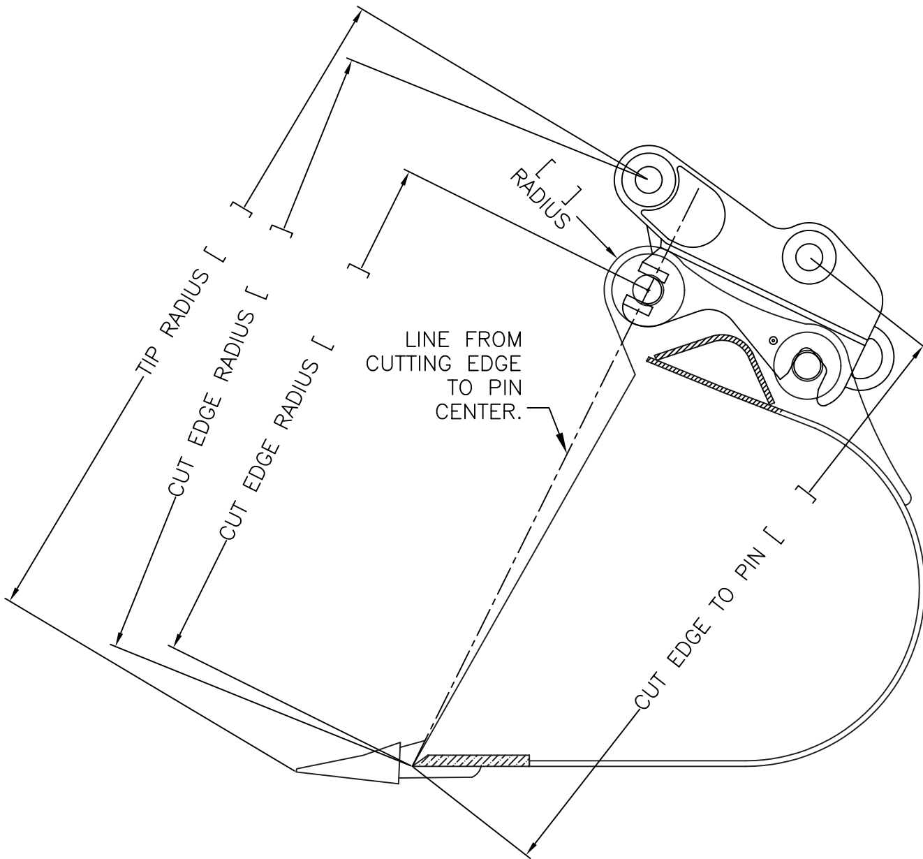
BUCKET RIGHT SIDE VIEW
